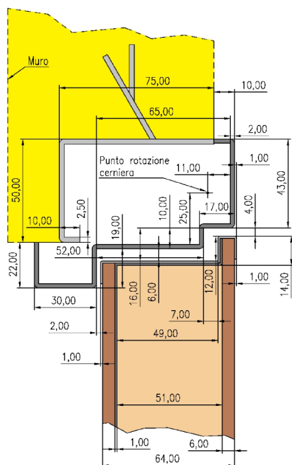
Profili anta, telaio e falso telaio Profile wing, frame and wrong frame
