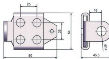
OCCHIOLI MOBILI ADJUSTABLE HASPS OEILLET MOBILE
